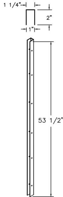
U CHANNEL (PILASTER/PANEL)
