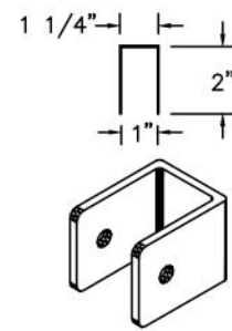
U BRACKET
