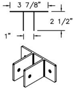
WALL BRACKET
