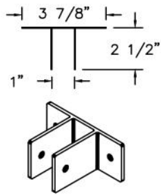
WALL BRACKET
