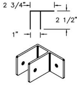
F BRACKET
