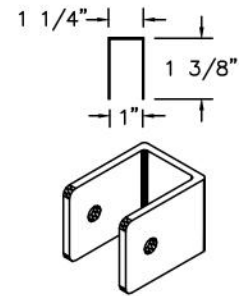
U BRACKET
