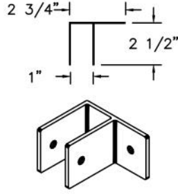
F BRACKET
