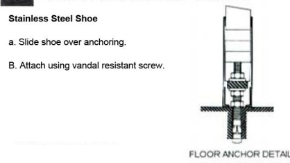
FLOOR ANCHOR DETAIL
