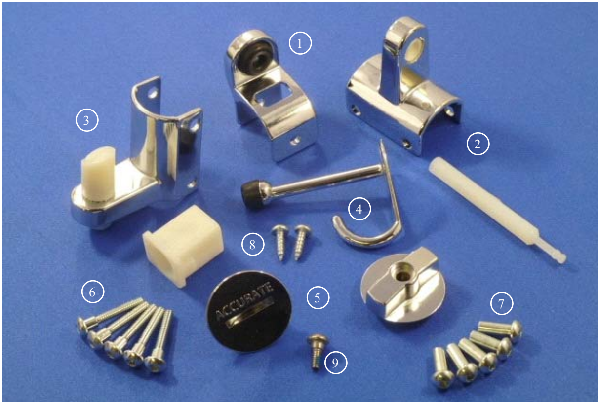
50-8511505 STD HARDWARE KIT GRAVITY HINGE—CHROME PLATED 50-8261505 STD HARDWARE KIT GRAVITY HINGE—STAINLESS STEEL
