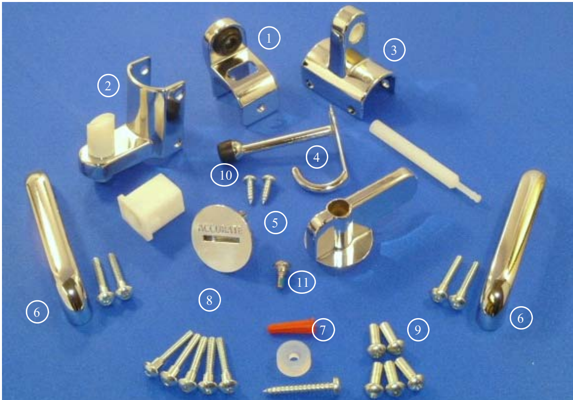
50-8511515 ADA HARDWARE KIT GRAVITY HINGE—CHROME PLATED 50-8261515 ADA HARDWARE KIT GRAVITY HINGE—STAINLESS STEEL
